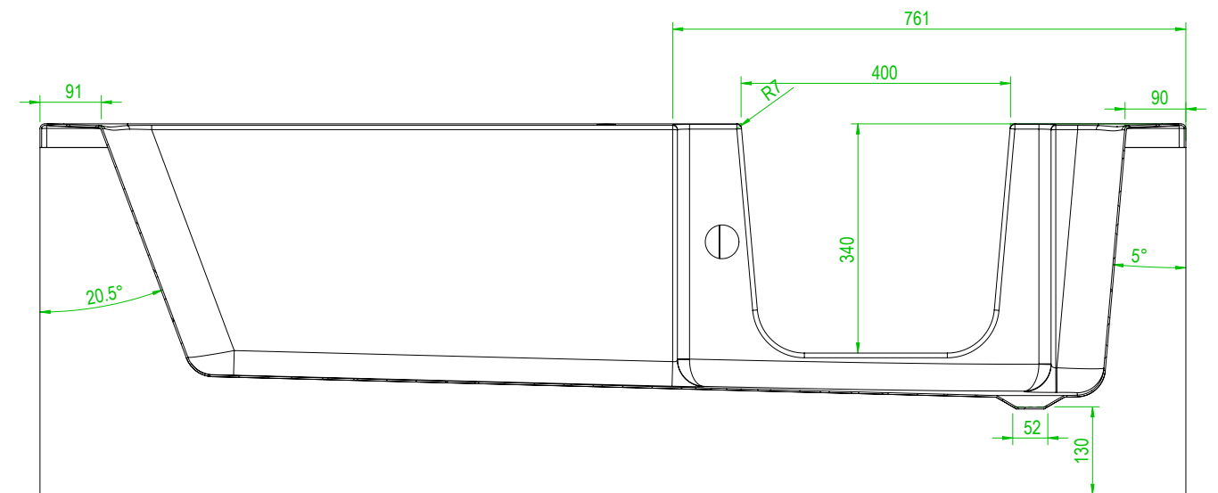
SECTION B-B
